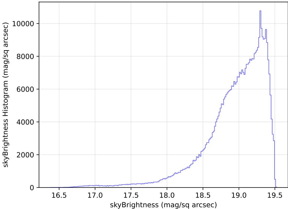
too_ignore_10_4v3.4_10yrs All sky z band: skyBrightness Histogram
