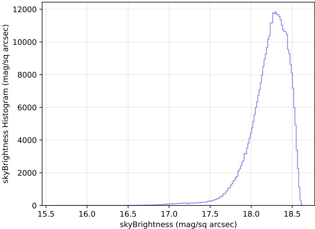
too_ignore_10_4v3.4_10yrs All sky y band: skyBrightness Histogram
