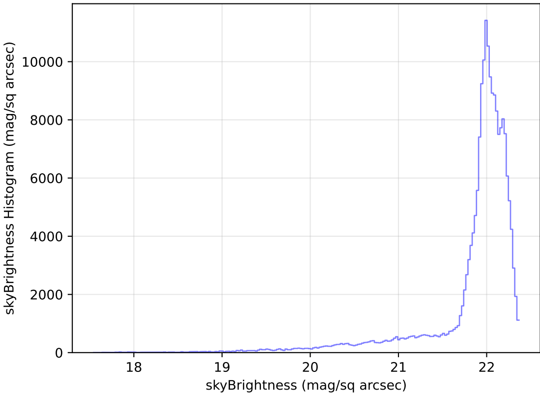
too_ignore_10_4v3.4_10yrs All sky g band: skyBrightness Histogram
