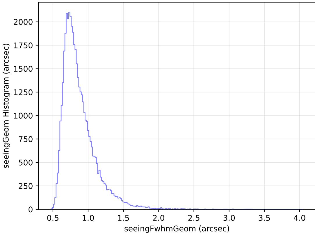
too_ignore_10_4v3.4_10yrs Yr 1 z band: seeingGeom Histogram
