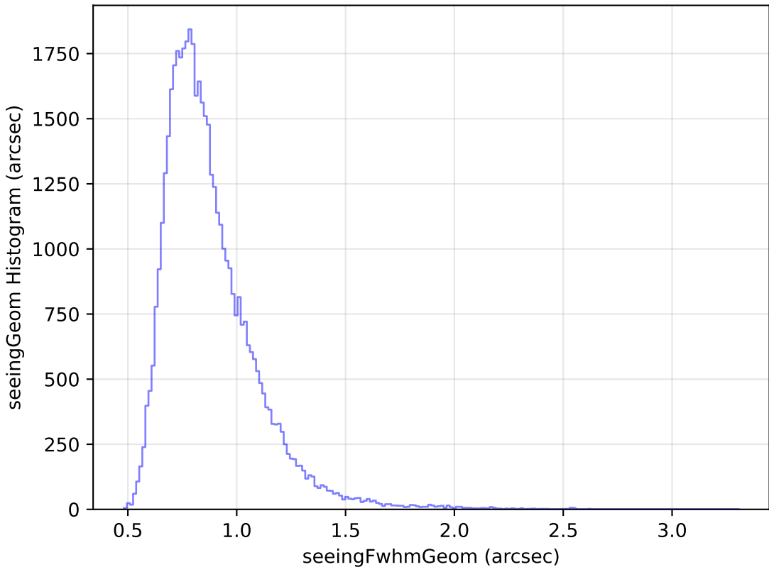
too_ignore_10_4v3.4_10yrs Yr 1 y band: seeingGeom Histogram
