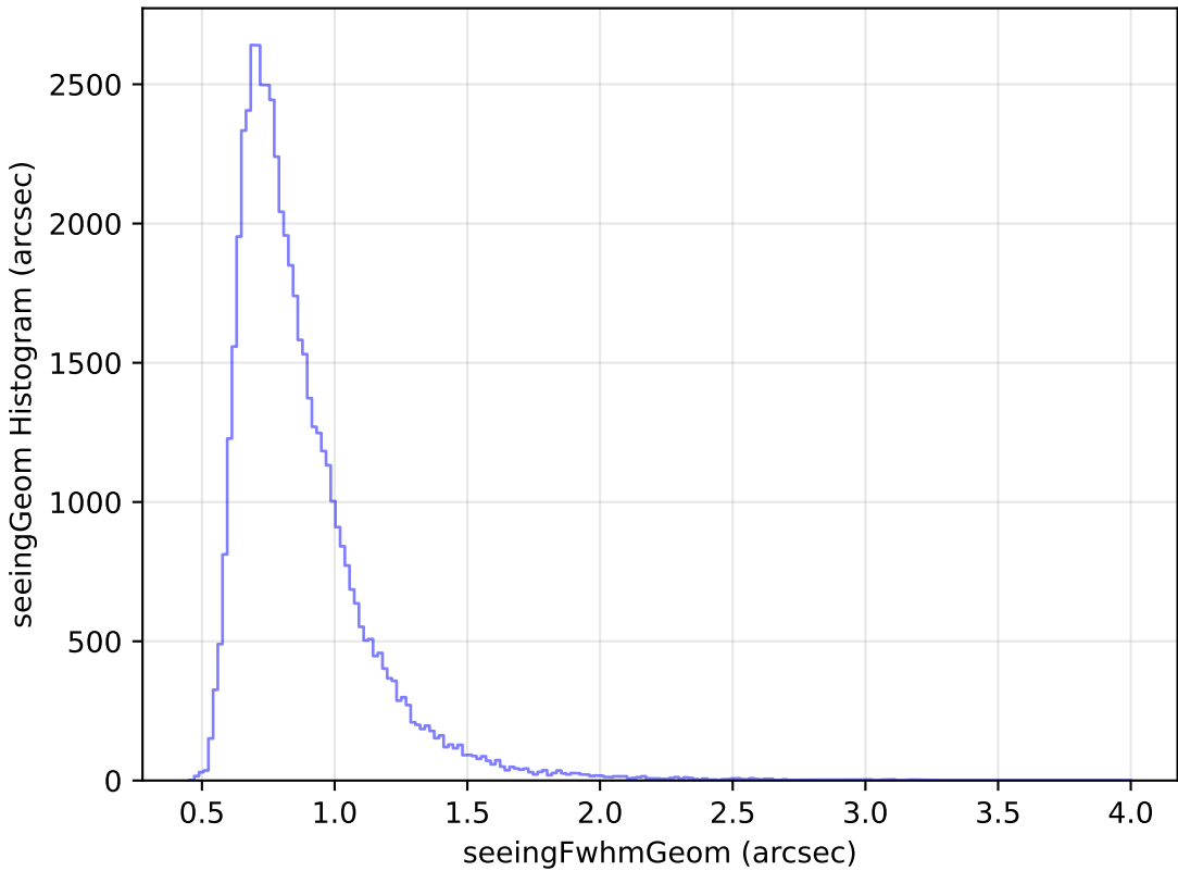
too_ignore_10_4v3.4_10yrs Yr 1 i band: seeingGeom Histogram
