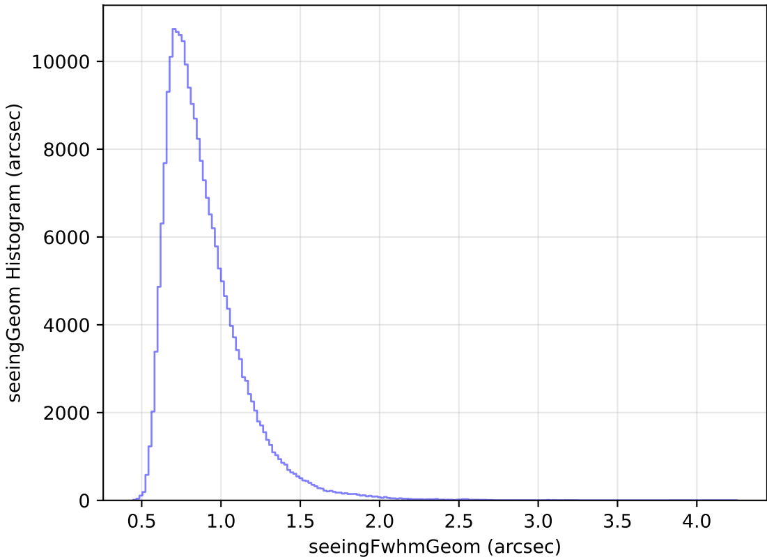
too_ignore_10_4v3.4_10yrs Yr 1 all bands: seeingGeom Histogram
