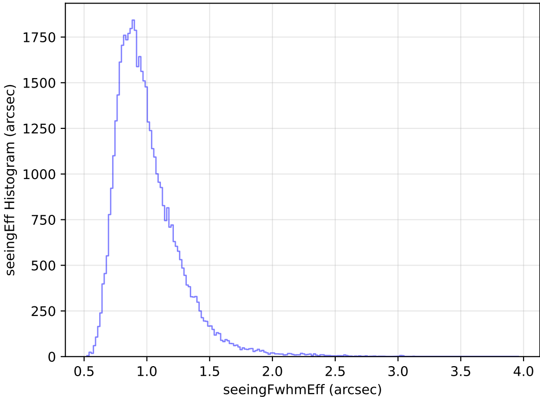
too_ignore_10_4v3.4_10yrs Yr 1 y band: seeingEff Histogram
