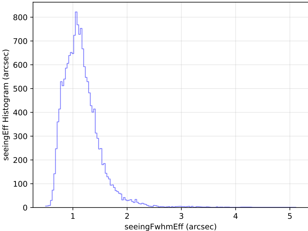
too_ignore_10_4v3.4_10yrs Yr 1 u band: seeingEff Histogram
