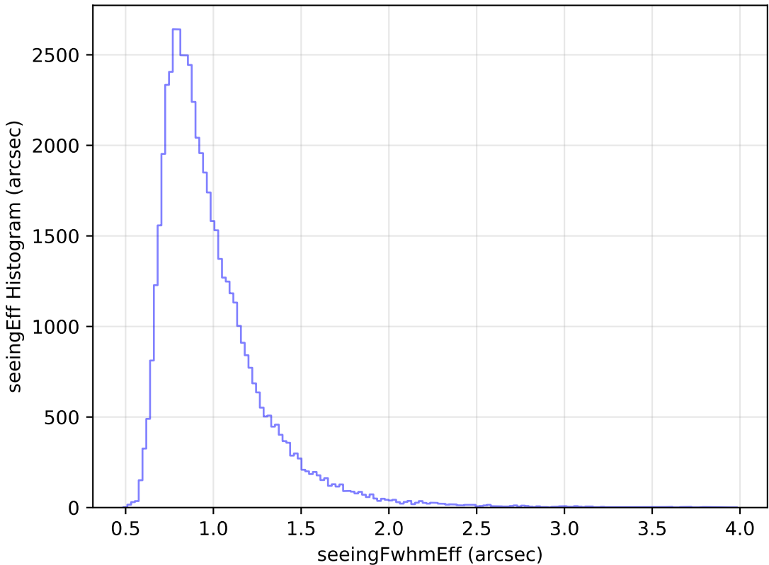
too_ignore_10_4v3.4_10yrs Yr 1 i band: seeingEff Histogram
