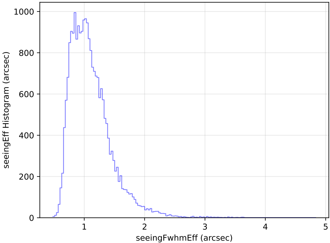
too_ignore_10_4v3.4_10yrs Yr 1 g band: seeingEff Histogram
