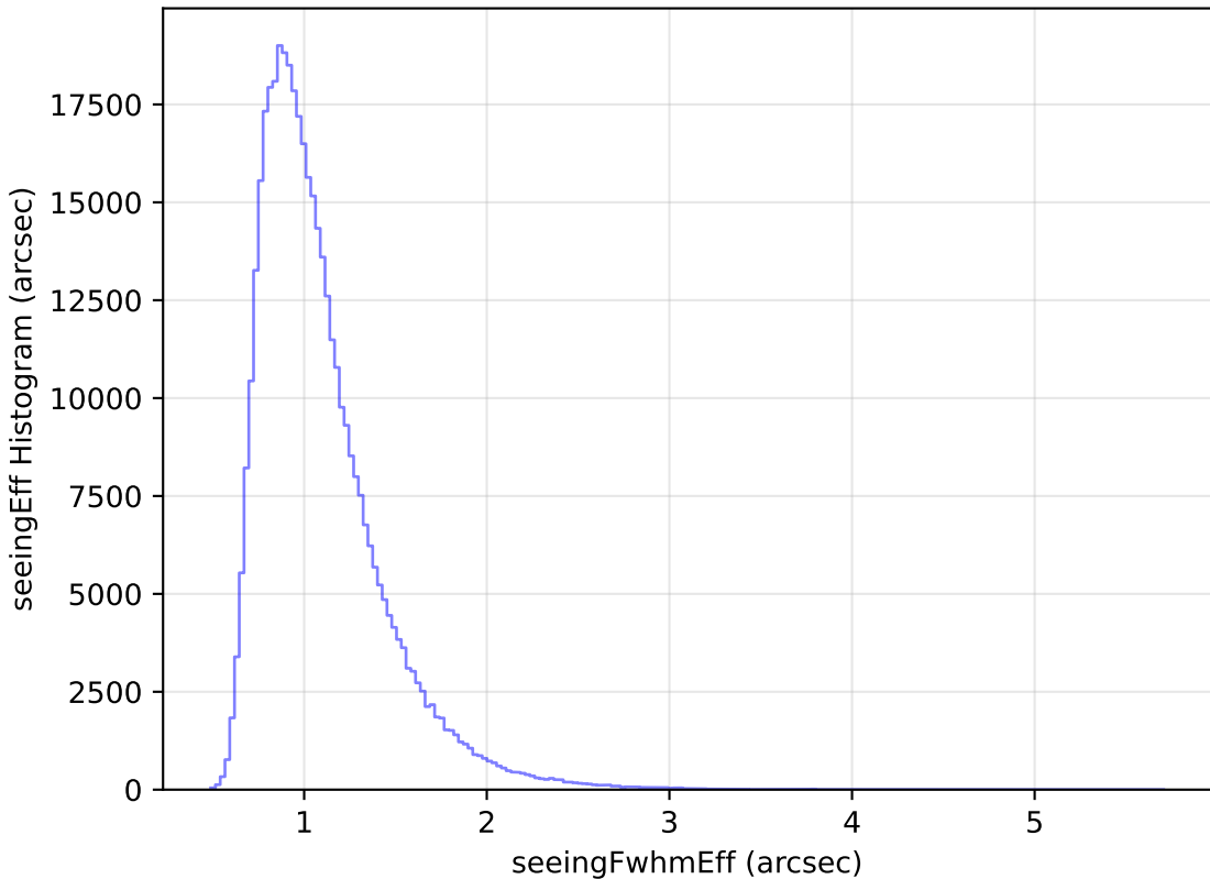
too_ignore_10_4v3.4_10yrs WFD z band: seeingEff Histogram
