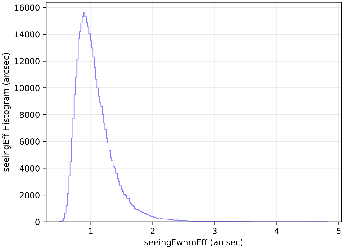
too_ignore_10_4v3.4_10yrs WFD y band: seeingEff Histogram
