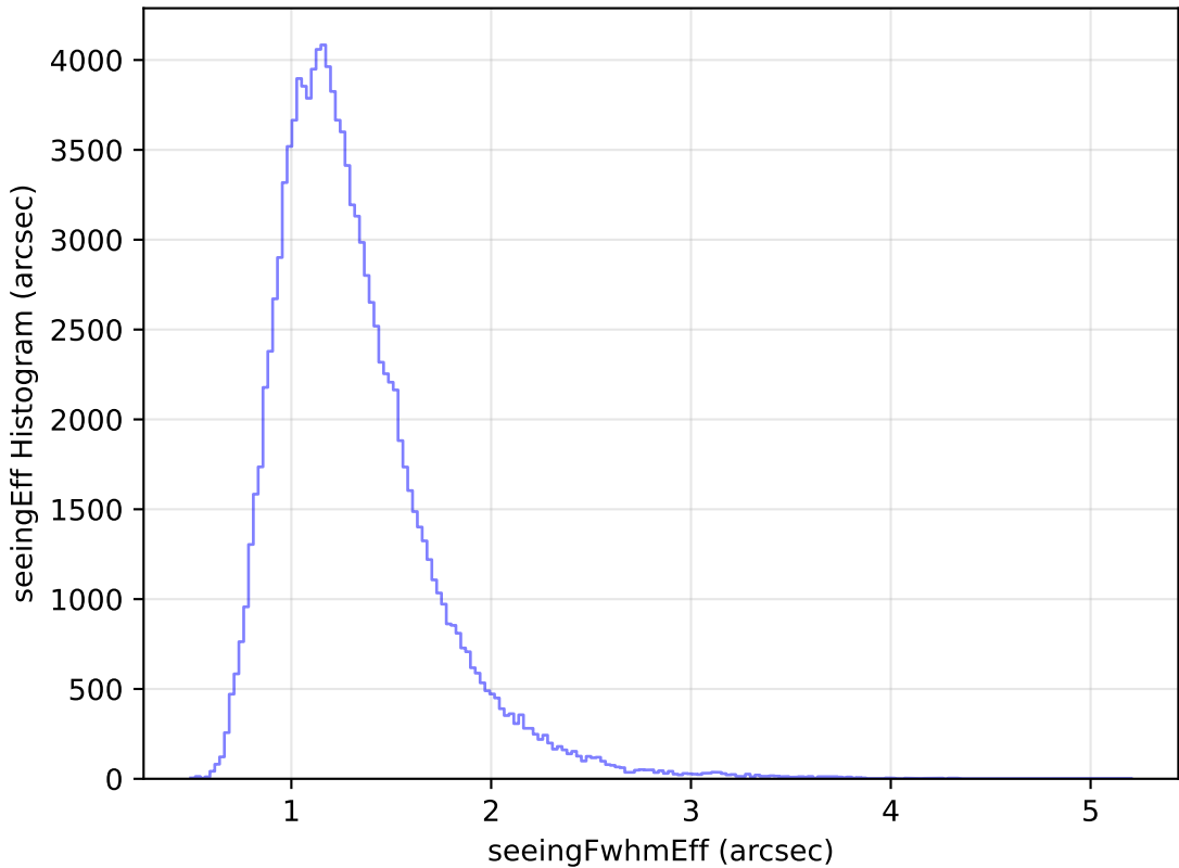
too_ignore_10_4v3.4_10yrs WFD u band: seeingEff Histogram
