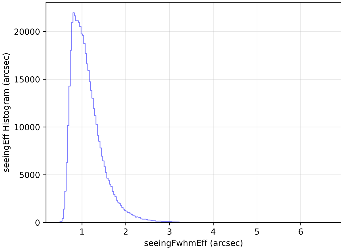
too_ignore_10_4v3.4_10yrs WFD r band: seeingEff Histogram
