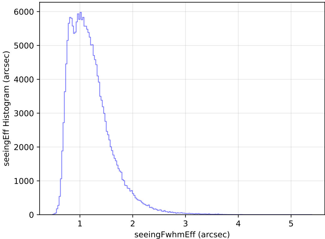
too_ignore_10_4v3.4_10yrs WFD g band: seeingEff Histogram
