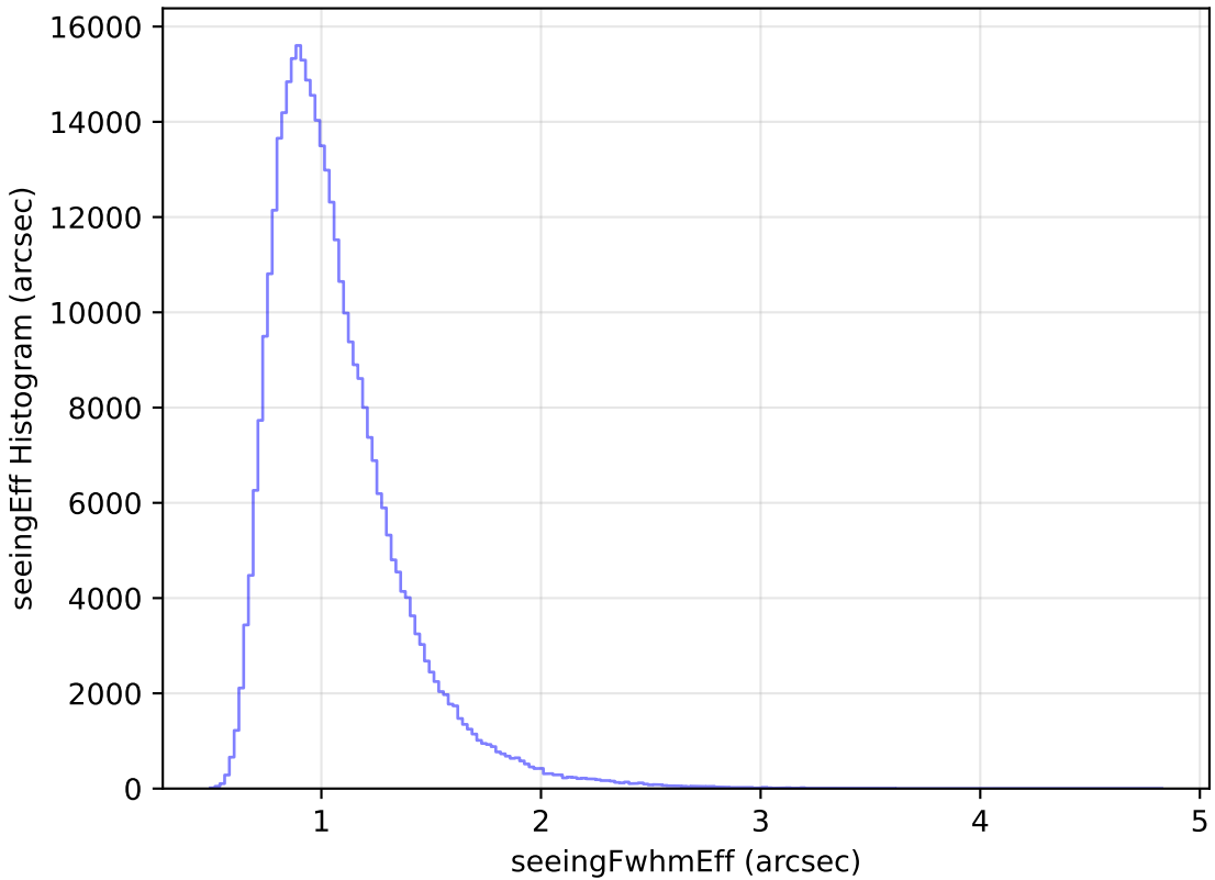
too_ignore_10_4v3.4_10yrs All sky y band: seeingEff Histogram
