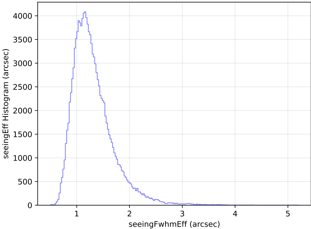
too_ignore_10_4v3.4_10yrs All sky u band: seeingEff Histogram
