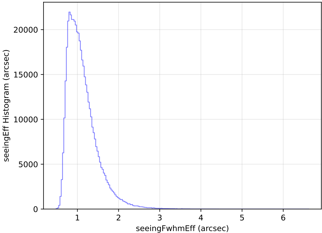
too_ignore_10_4v3.4_10yrs All sky r band: seeingEff Histogram
