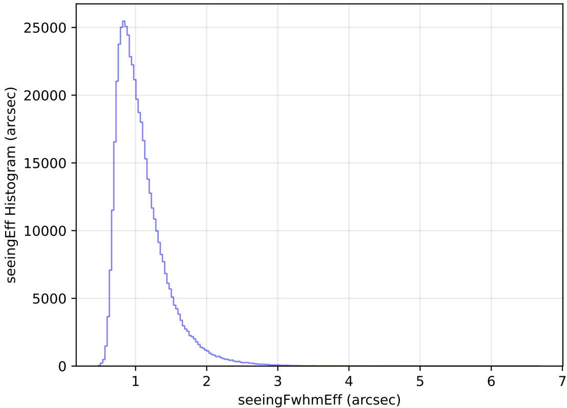
too_ignore_10_4v3.4_10yrs All sky i band: seeingEff Histogram
