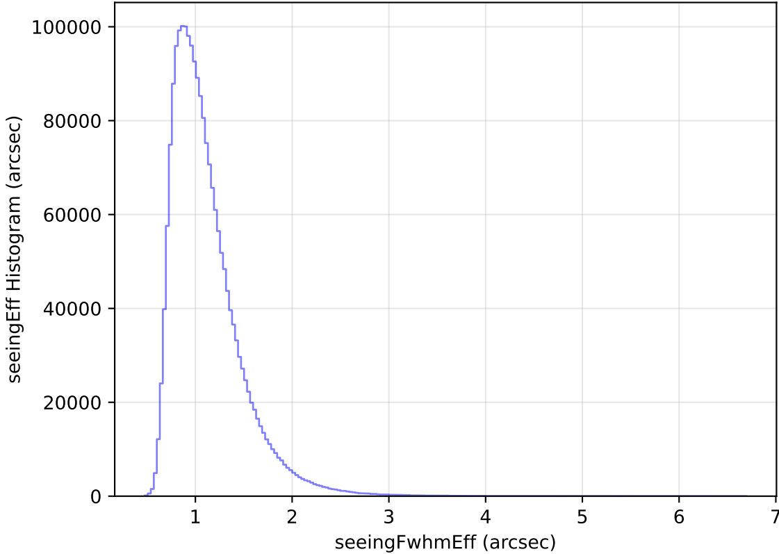
too_ignore_10_4v3.4_10yrs All sky all bands: seeingEff Histogram
