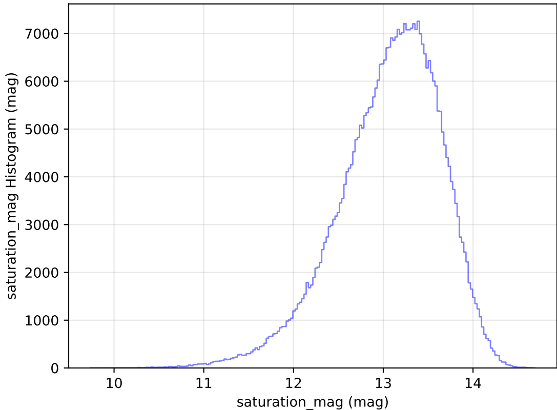
too_ignore_10_4v3.4_10yrs WFD y band: saturation_mag Histogram
