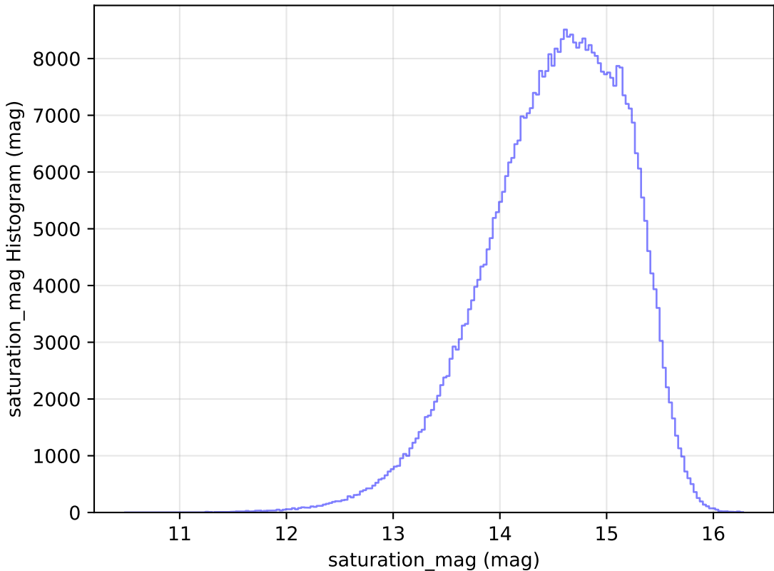
too_ignore_10_4v3.4_10yrs WFD r band: saturation_mag Histogram
