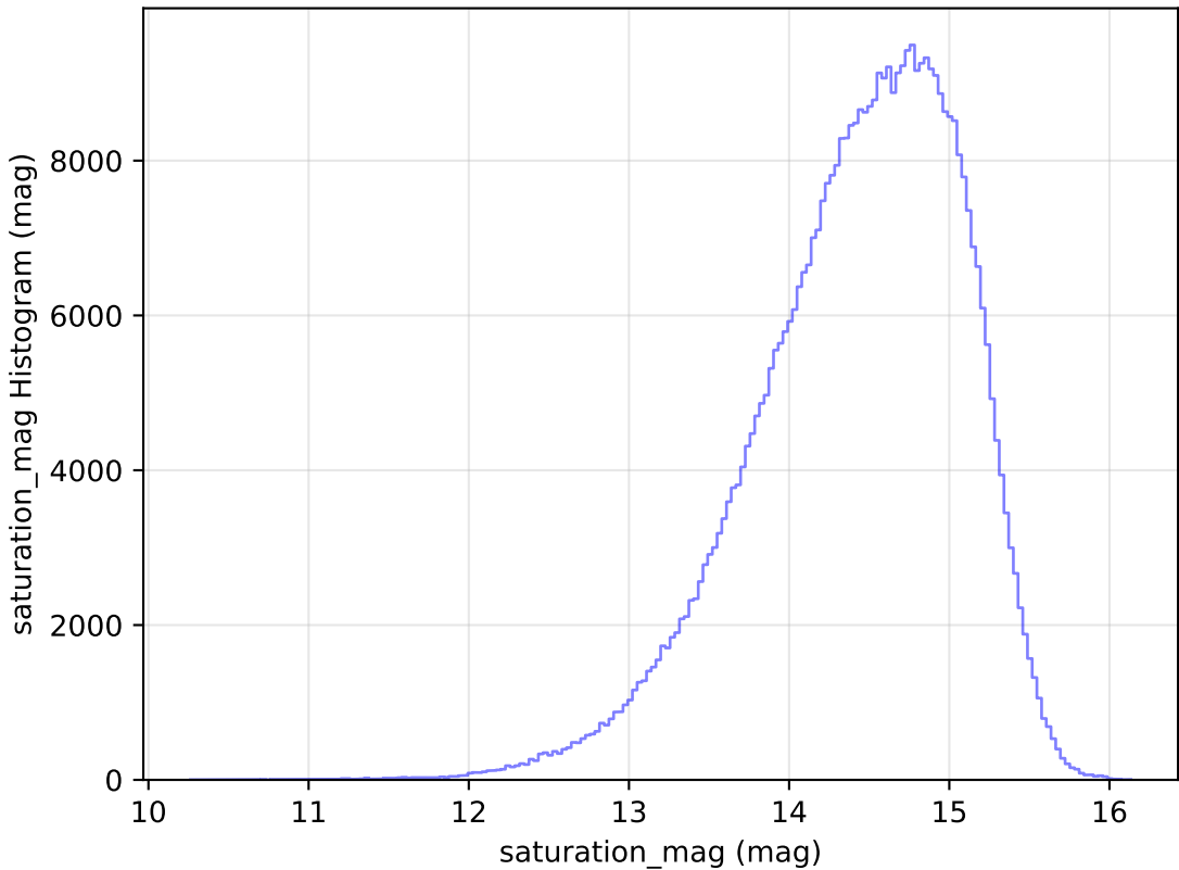
too_ignore_10_4v3.4_10yrs WFD i band: saturation_mag Histogram
