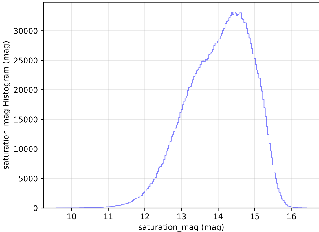
too_ignore_10_4v3.4_10yrs WFD all bands: saturation_mag Histogram
