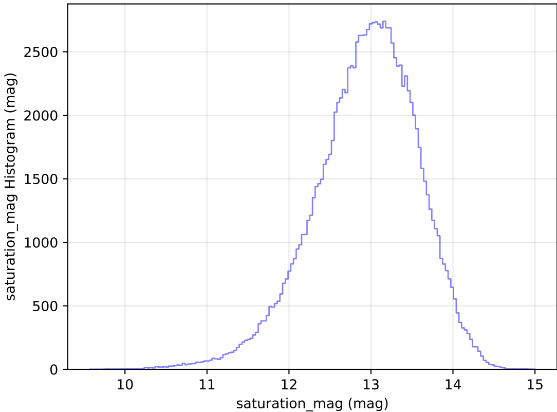
too_ignore_10_4v3.4_10yrs All sky u band: saturation_mag Histogram
