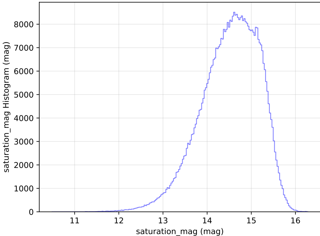
too_ignore_10_4v3.4_10yrs All sky r band: saturation_mag Histogram
