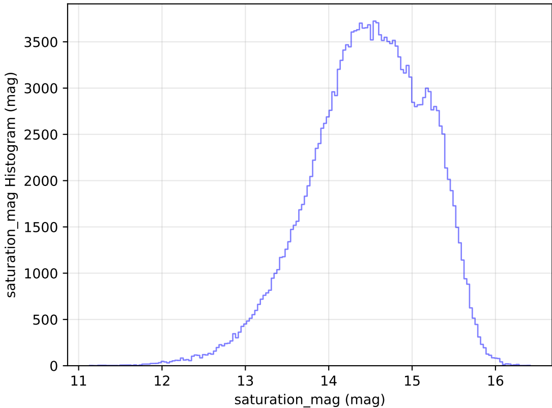
too_ignore_10_4v3.4_10yrs All sky g band: saturation_mag Histogram
