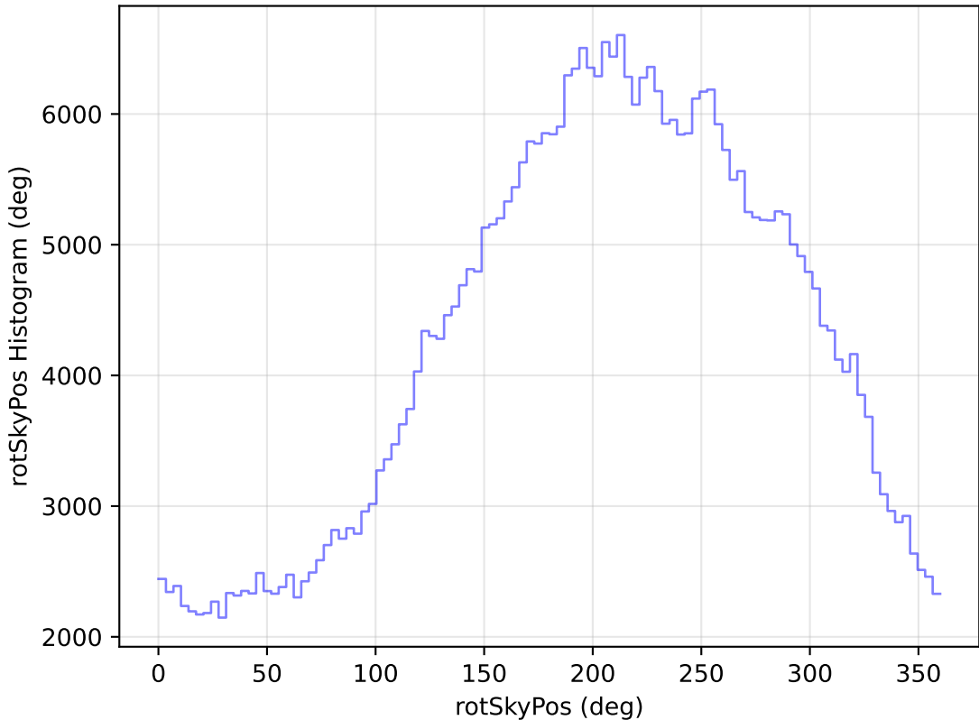
too_ignore_10_4v3.4_10yrs WFD z band: rotSkyPos Histogram
