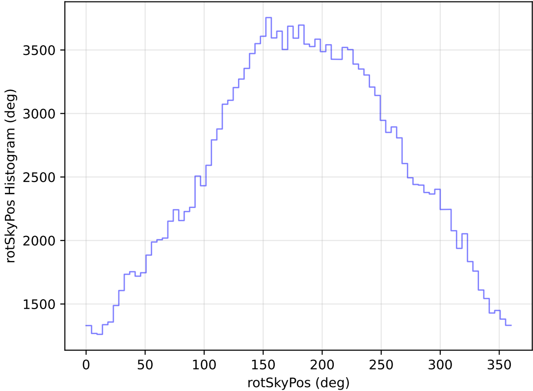
too_ignore_10_4v3.4_10yrs WFD g band: rotSkyPos Histogram
