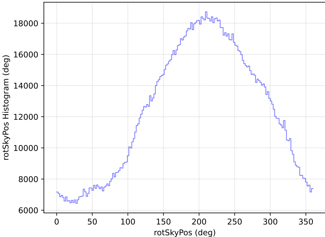
too_ignore_10_4v3.4_10yrs WFD all bands: rotSkyPos Histogram
