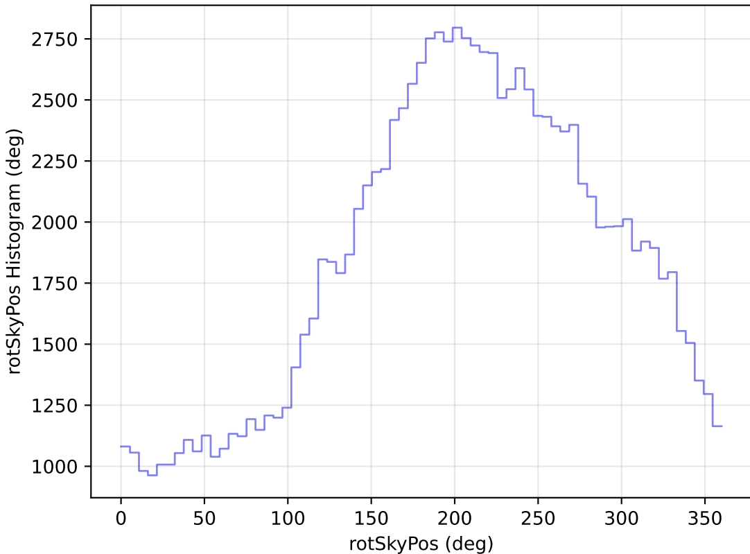
too_ignore_10_4v3.4_10yrs All sky u band: rotSkyPos Histogram
