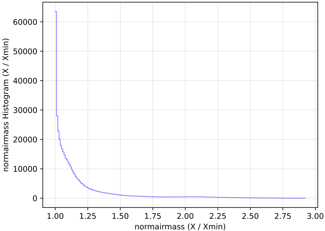
too_ignore_10_4v3.4_10yrs WFD z band: normairmass Histogram
