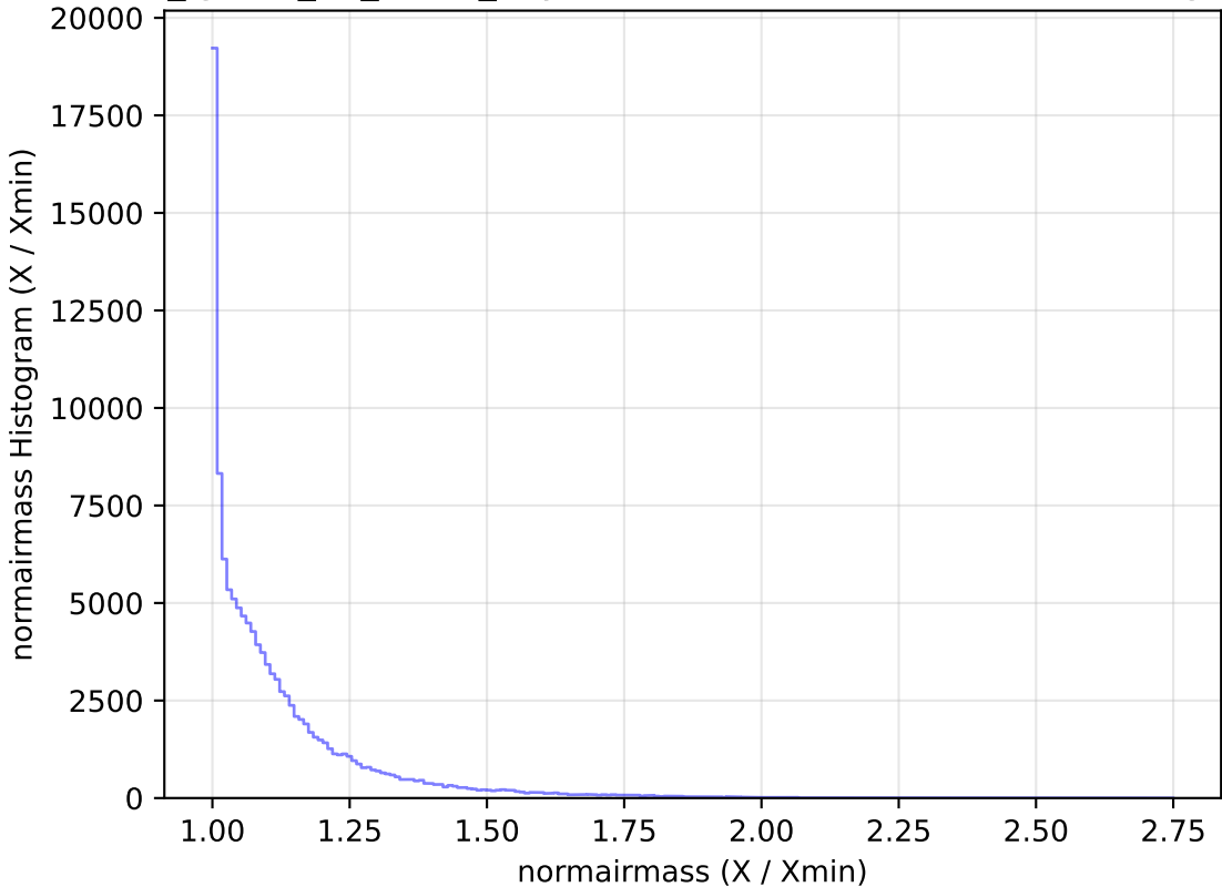
too_ignore_10_4v3.4_10yrs WFD u band: normairmass Histogram
