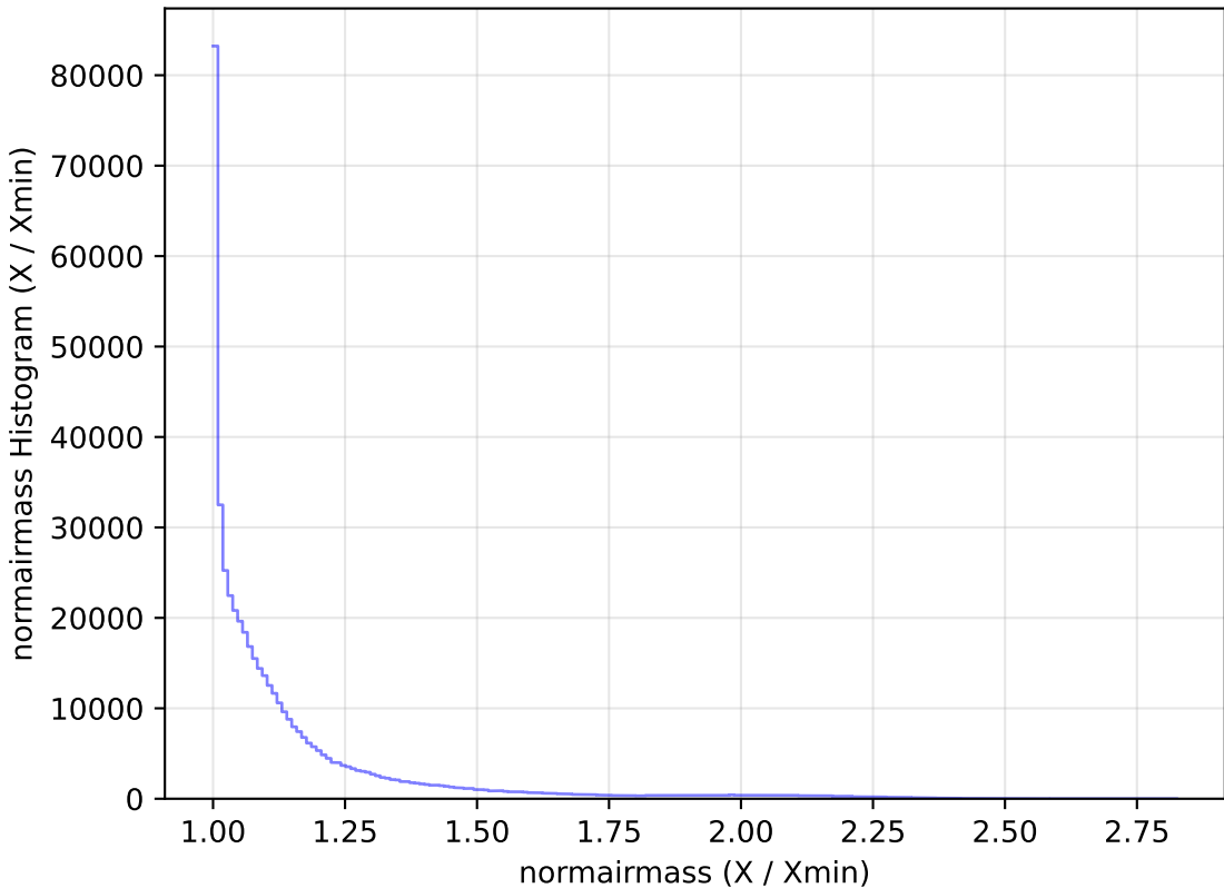
too_ignore_10_4v3.4_10yrs WFD r band: normairmass Histogram
