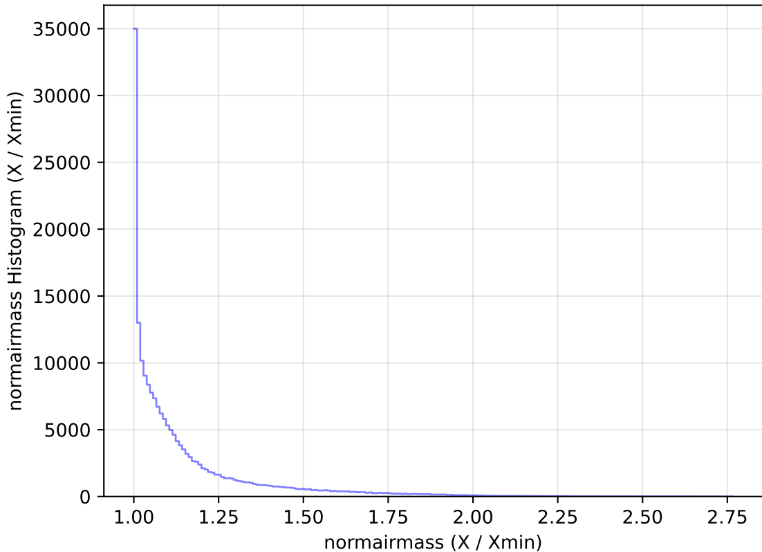
too_ignore_10_4v3.4_10yrs WFD g band: normairmass Histogram
