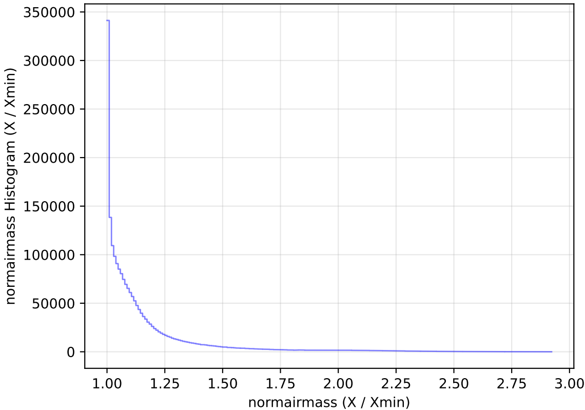
too_ignore_10_4v3.4_10yrs WFD all bands: normairmass Histogram
