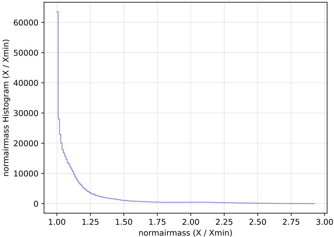
too_ignore_10_4v3.4_10yrs All sky z band: normairmass Histogram
