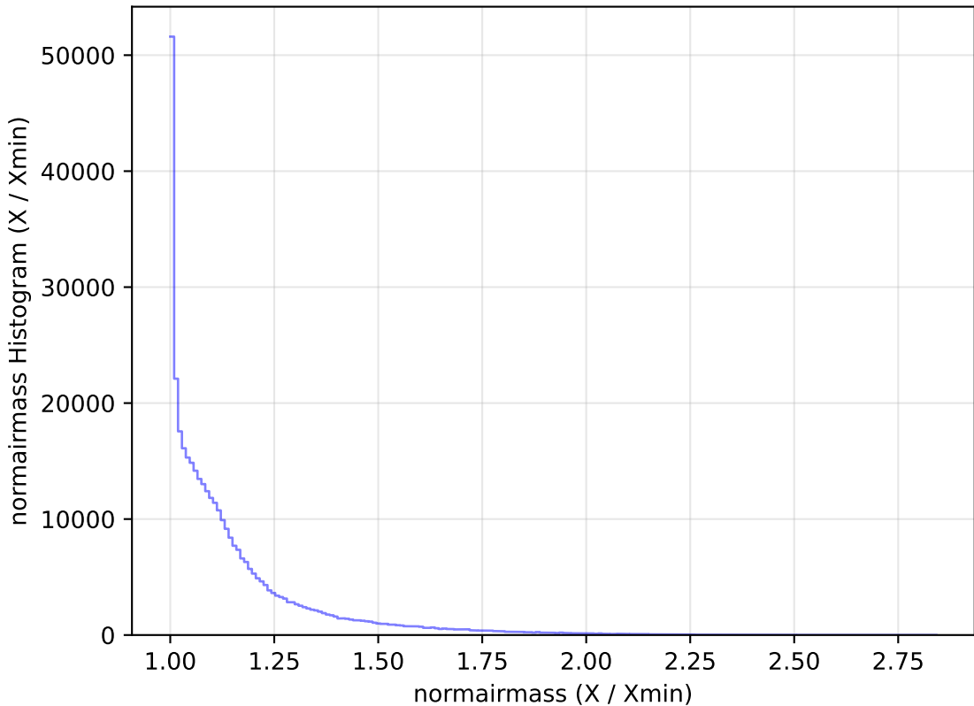
too_ignore_10_4v3.4_10yrs All sky y band: normairmass Histogram
