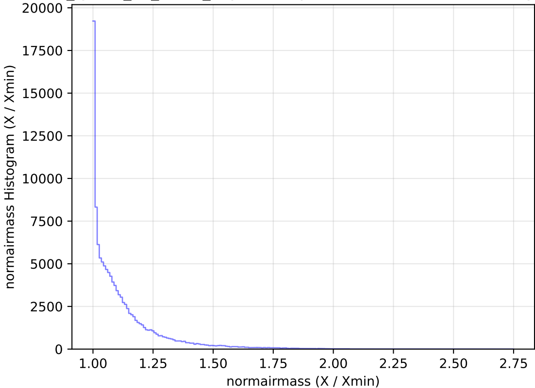
too_ignore_10_4v3.4_10yrs All sky u band: normairmass Histogram
