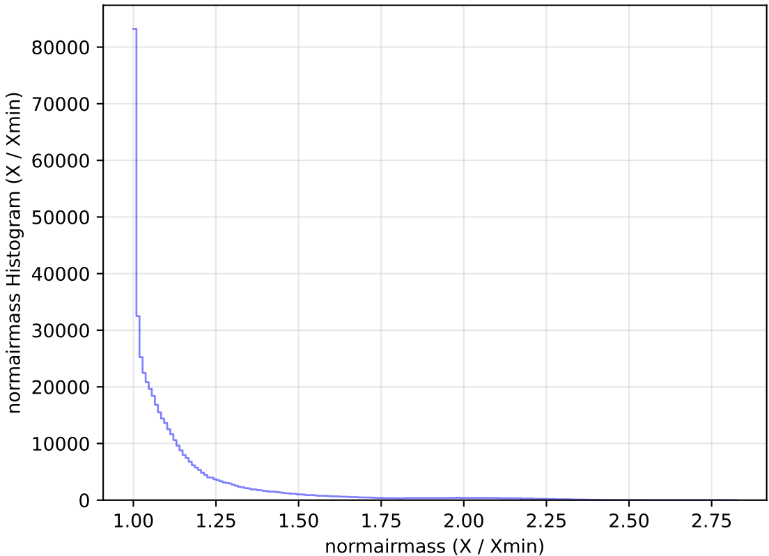
too_ignore_10_4v3.4_10yrs All sky r band: normairmass Histogram
