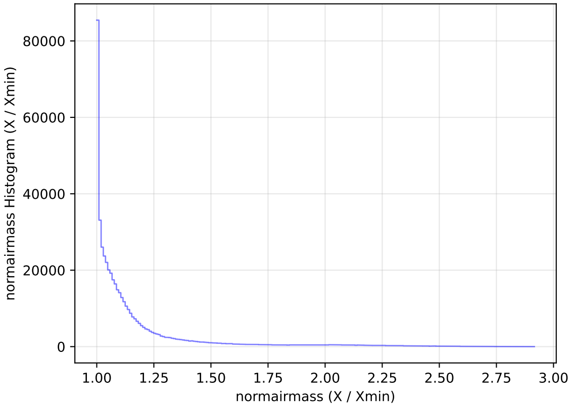
too_ignore_10_4v3.4_10yrs All sky i band: normairmass Histogram
