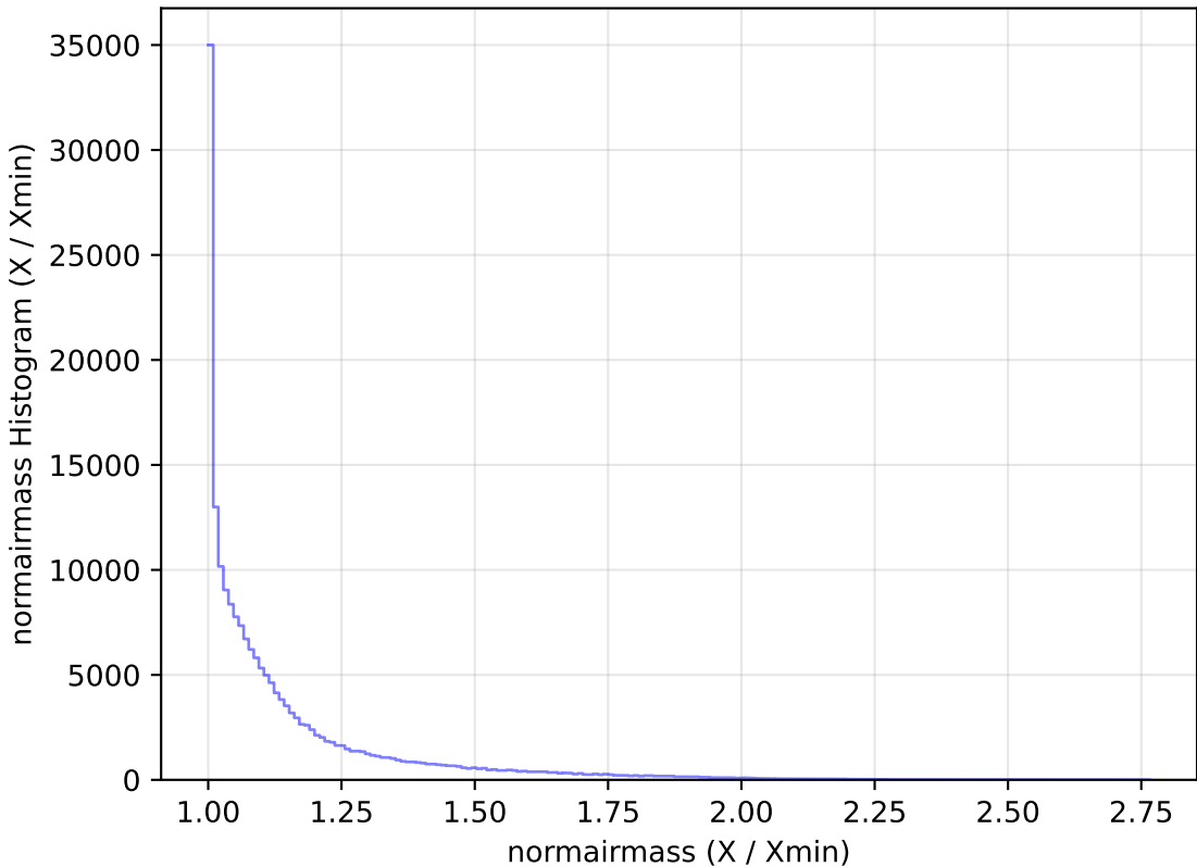
too_ignore_10_4v3.4_10yrs All sky g band: normairmass Histogram
