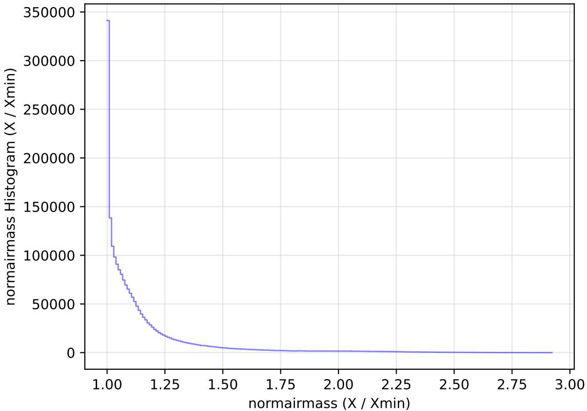
too_ignore_10_4v3.4_10yrs All sky all bands: normairmass Histogram
