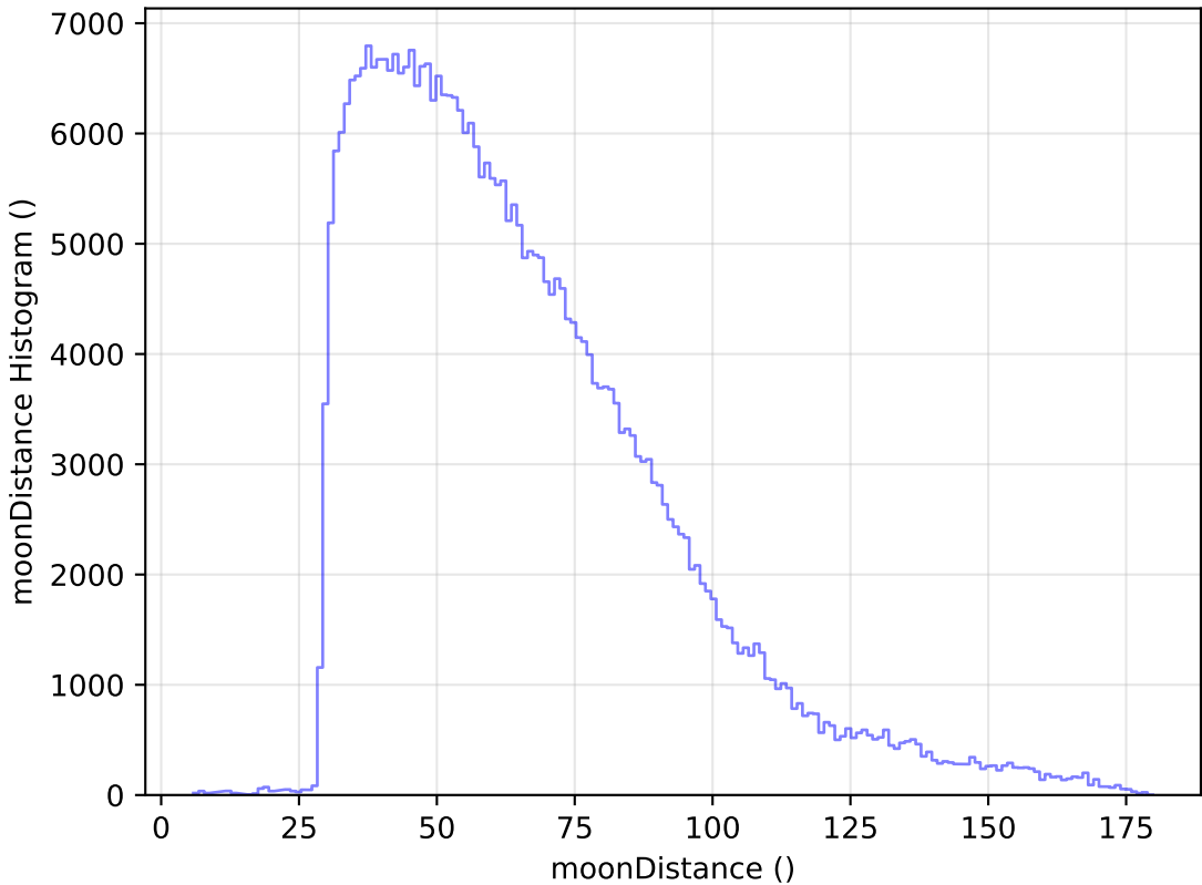
too_ignore_10_4v3.4_10yrs WFD y band: moonDistance Histogram
