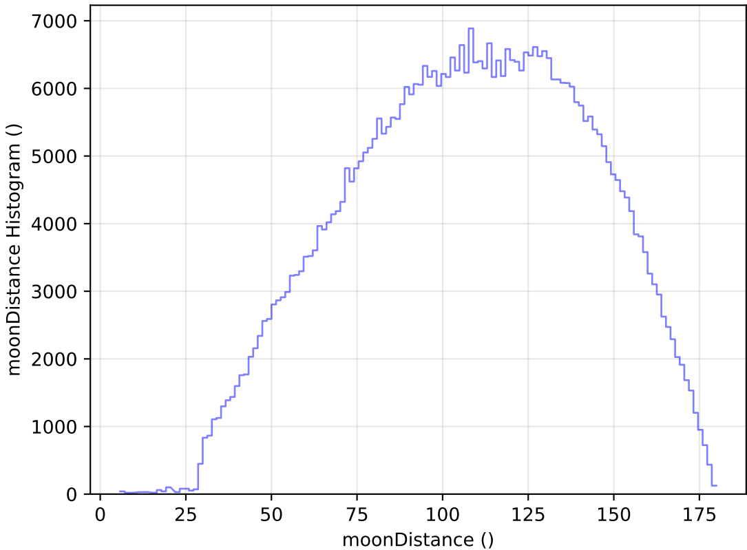
too_ignore_10_4v3.4_10yrs WFD r band: moonDistance Histogram
