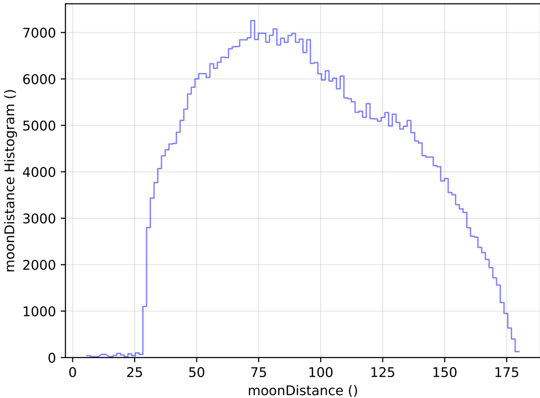
too_ignore_10_4v3.4_10yrs WFD i band: moonDistance Histogram
