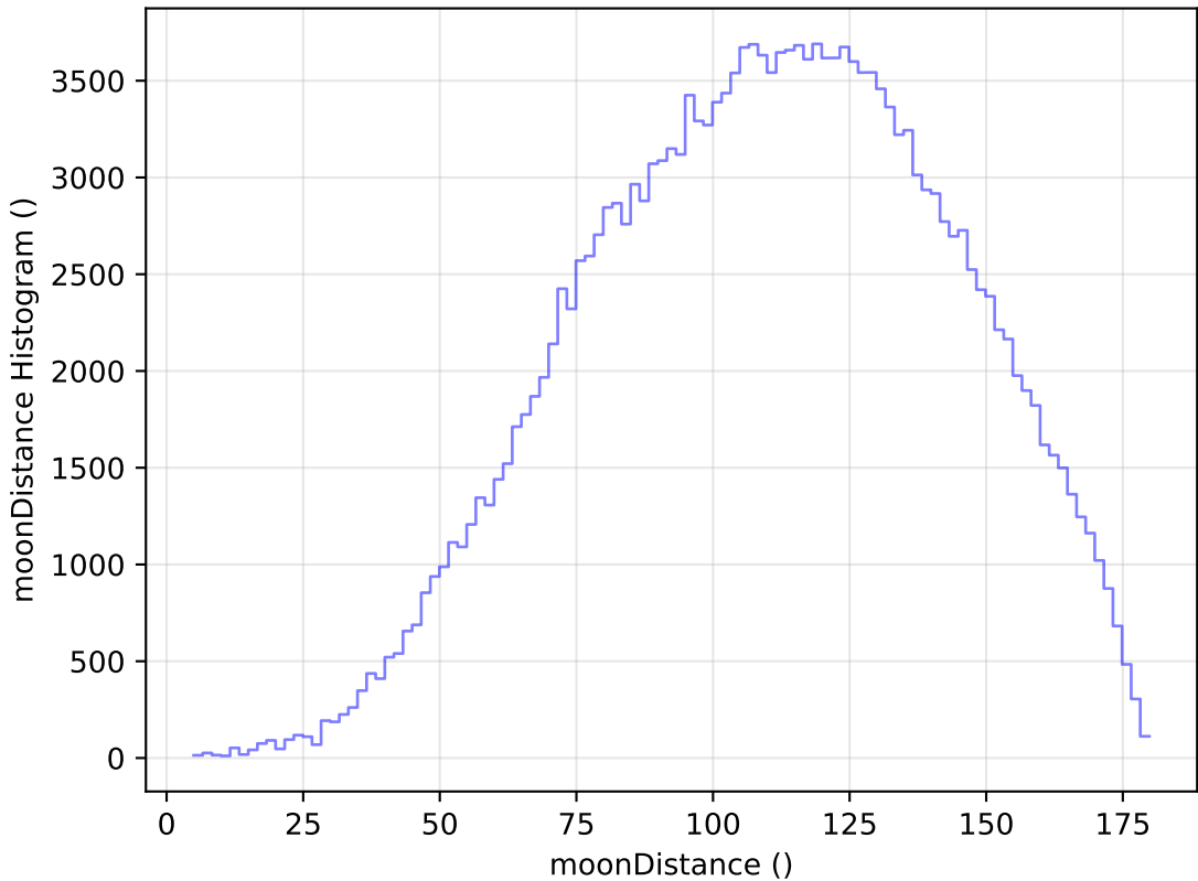
too_ignore_10_4v3.4_10yrs WFD g band: moonDistance Histogram
