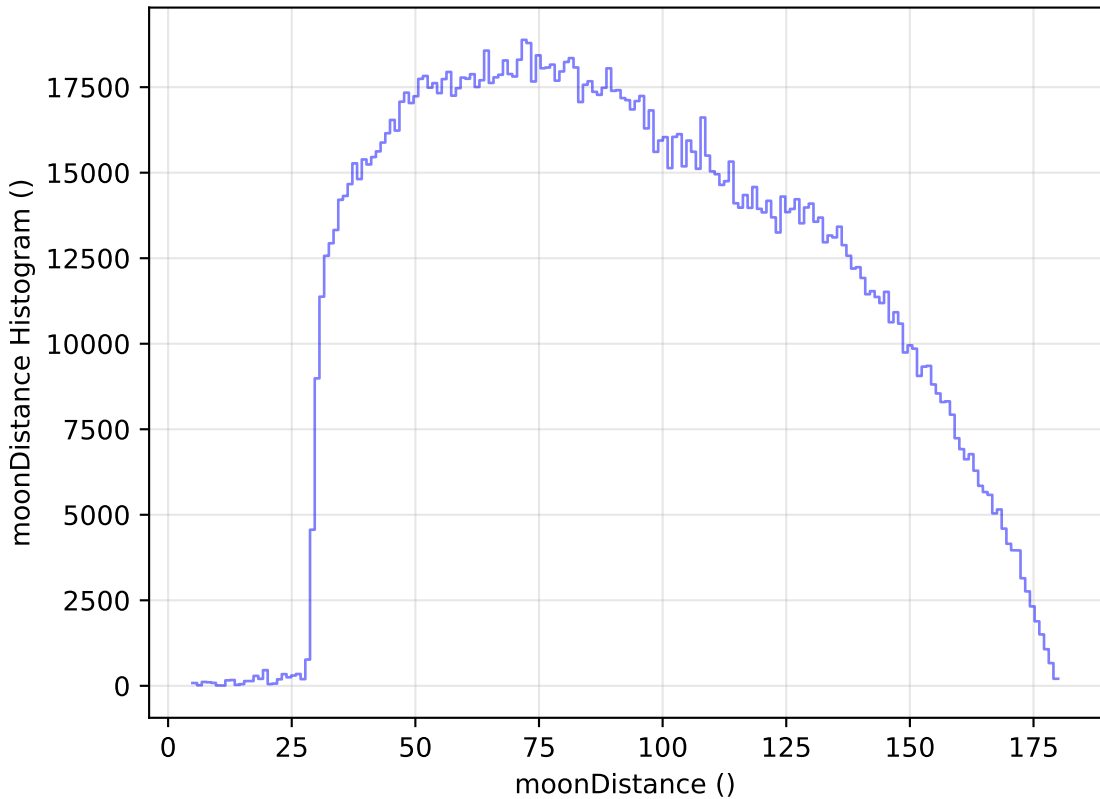
too_ignore_10_4v3.4_10yrs WFD all bands: moonDistance Histogram
