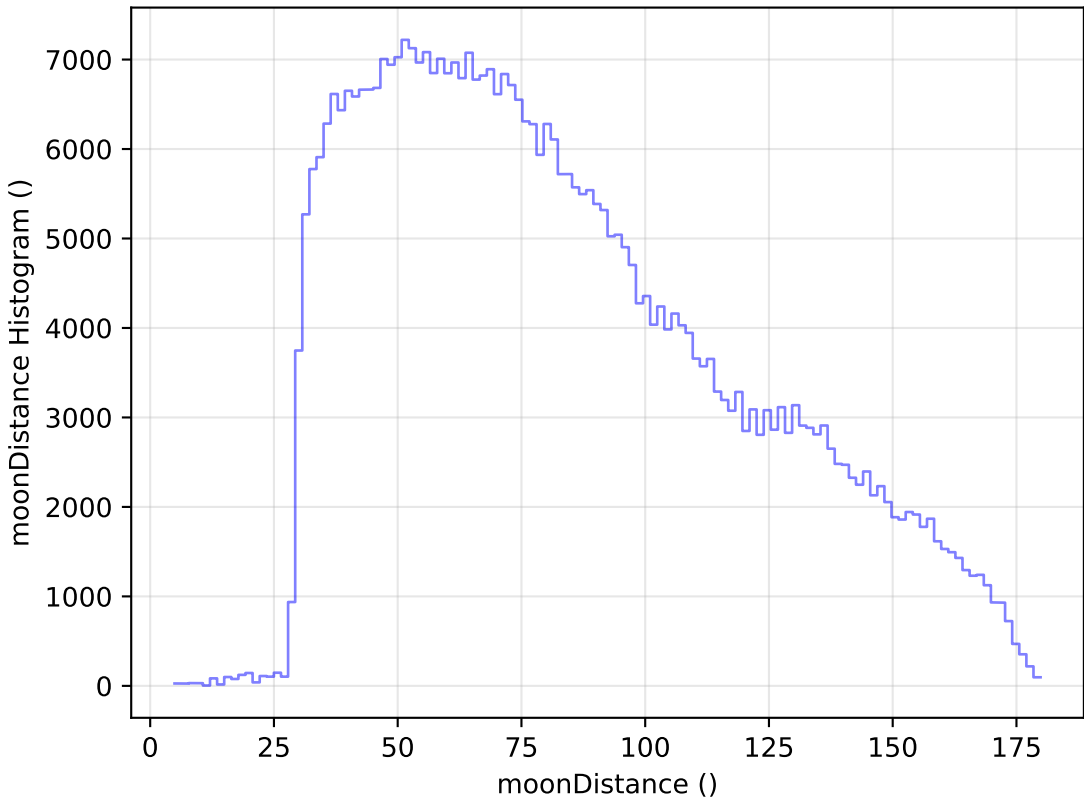
too_ignore_10_4v3.4_10yrs All sky z band: moonDistance Histogram
